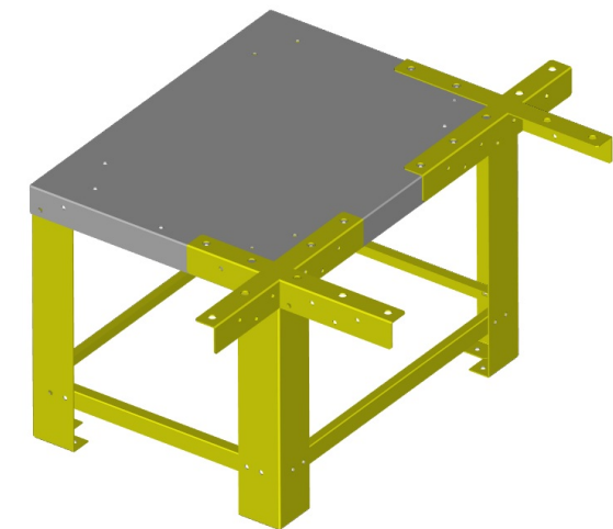
Assembled Stand - Possible Positions for CABLE SUPPORT BAR
